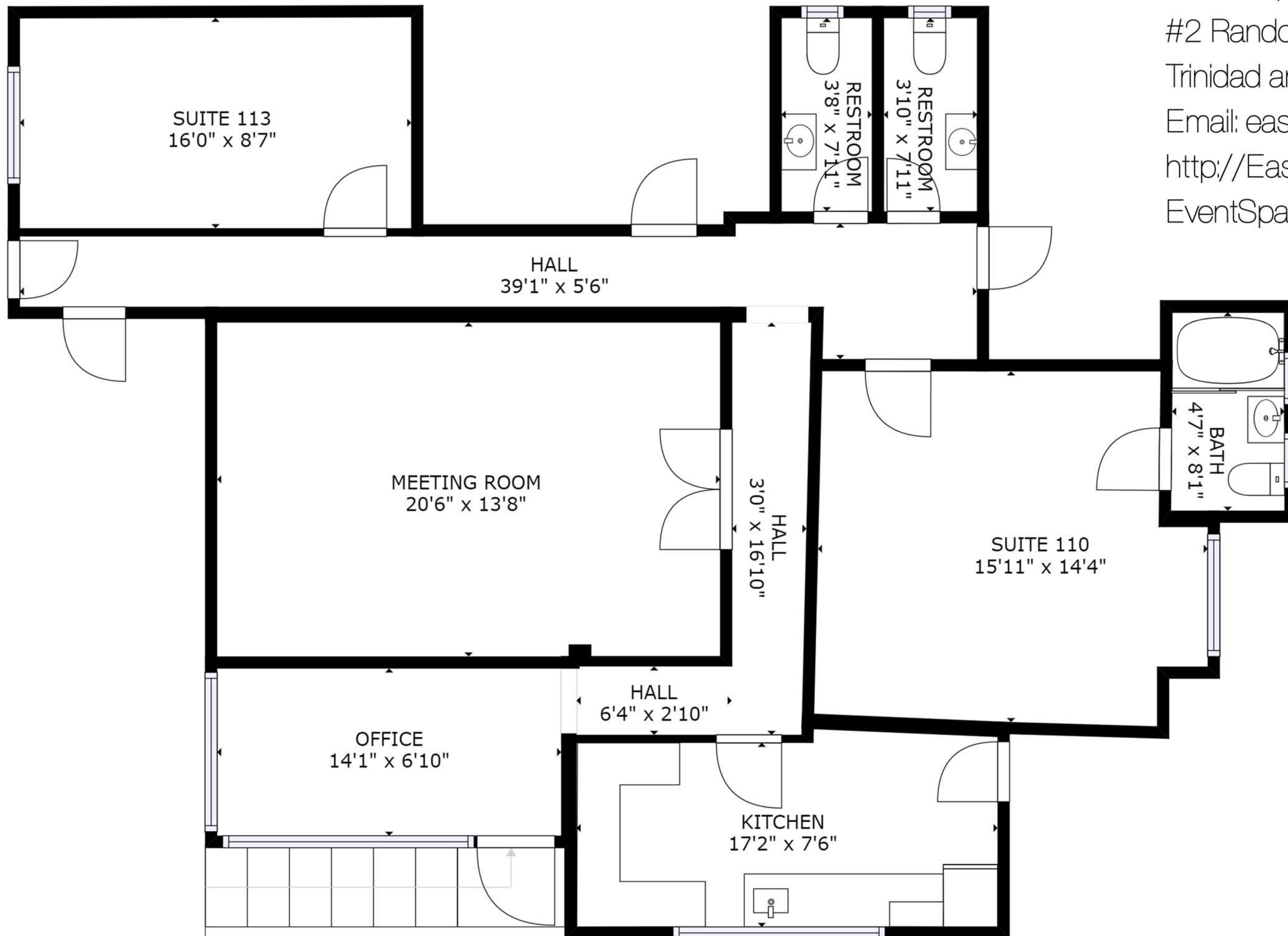
FLOOR 1
